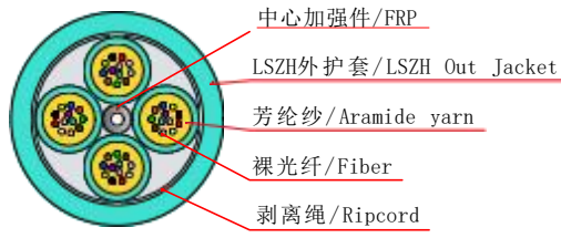
Optical cable Diagram
